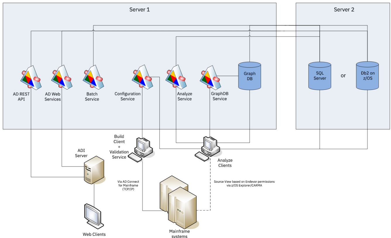
Figure 1. IBM AD high-level architecture
